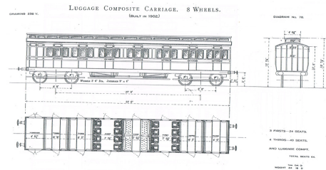
Diagram 78 Luggage Composite
