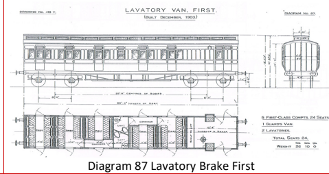
Diagram 87 Lavatory Brake First
