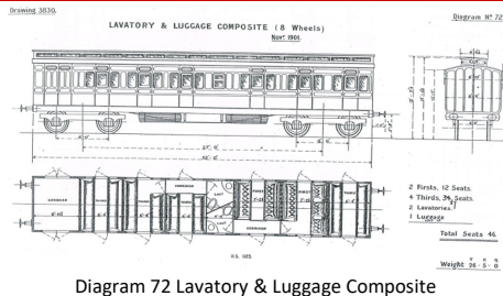
Diagram 72 Lavatory & Luggage Composite
