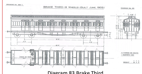
Diagram 83 Brake Third
