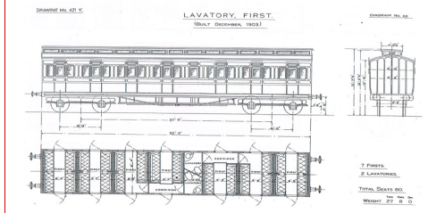
Diagram 86 Lavatory First
