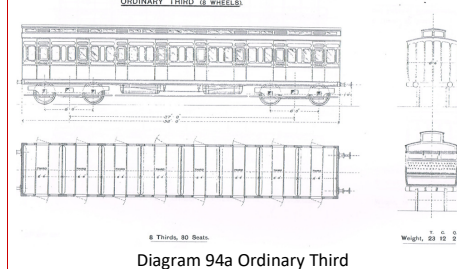
Diagram 94a Ordinary Third
