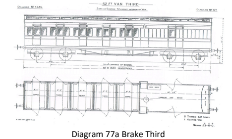
Diagram 77a Brake Third
