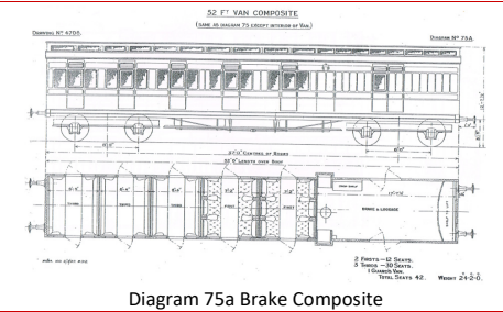
Diagram 75a Brake Composite
