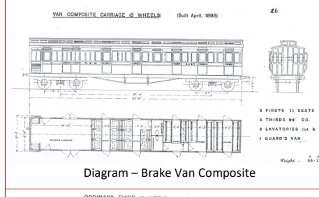
Diagram 89 Brake Composite
