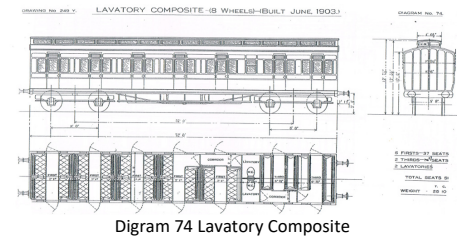
Diagram 74 Lavatory Composite
