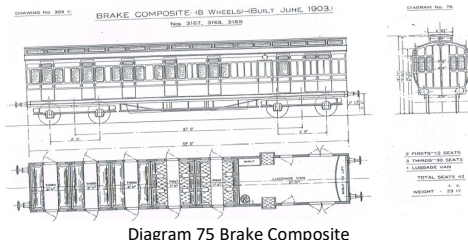
Diagram 75 Brake Composite
