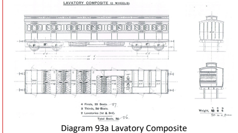
Diagram 93a Lavatory Composite
